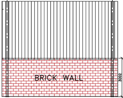
ELEVATION FOR GRID A
