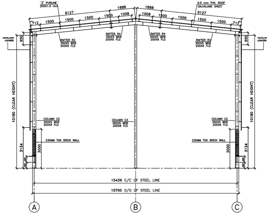
PORTAL FRAME AT GRID 1 & 2.
