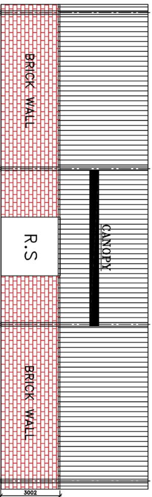
ELEVATION FOR GRID C
